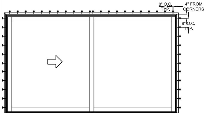
TYPICAL ELEVATION WITH FASTENER SPACING
